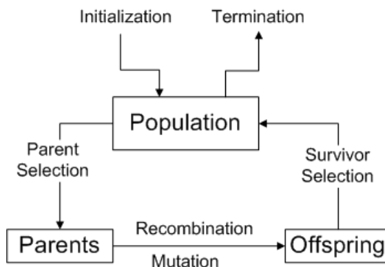
Figure 5.1: Evolution Cycle
