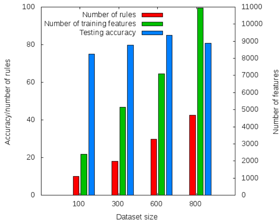
Figure 4.8: C4.5 Results
