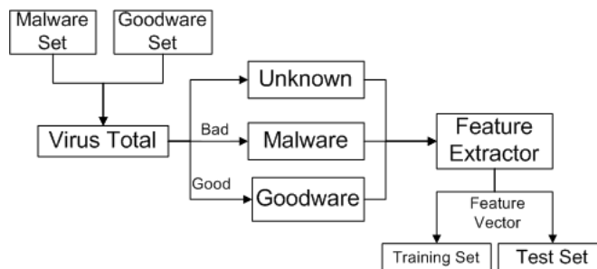
Figure 4.1: Pre-processing stage
